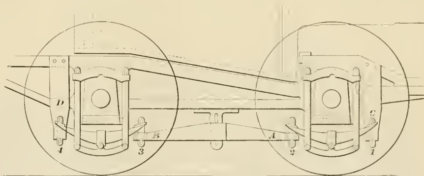
UNDERHUNG SPRINGS.
